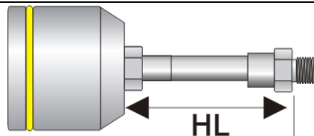
C1: HL=50mm
